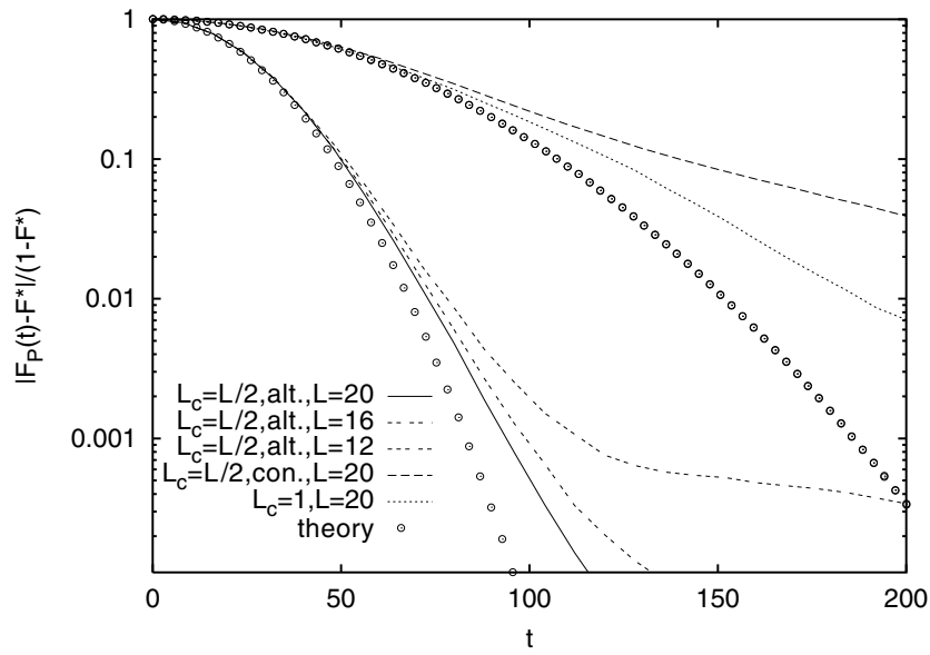
Figure 9. Same as in figure 8 but for the integrable regime (a). Note that the theoretical (Gaussian extrapolated) curves for cases (C, S) are practically indistinguishable.
