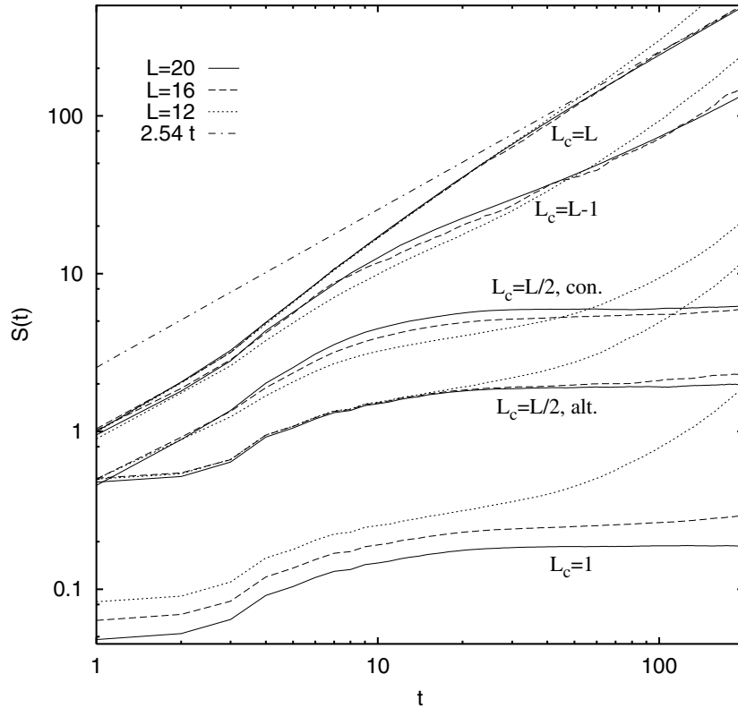
Figure 2. Partial correlation sums in the mixing regime h_z = 1.4 for different divisions \mathbb{Z}_L = \mathcal{J} \cup \mathcal{J}' . The structure (alternating A versus continuous C) and/or the number L_c of elements of the set \mathcal{J}' is indicated in the label near each triple of curves (full for L = 20 , dashed for L = 16 and dotted for L = 12 ).
