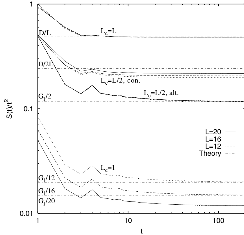
Figure 4. Partial correlation sums in the integrable regime h_z = 0.0 compared to the analytically computed coefficients for different divisions indicated by labels describing the structure (continuous/alternating) and number of elements of the set \mathcal{J}' .
