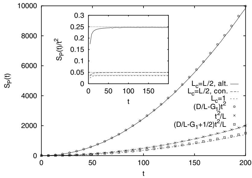
Figure 5. Purity correlator S_P(t) in the integrable regime h_z = 0.0 compared with analytical expressions (sampled symbols) for different cases of divisions (A, C, S). In the inset we emphasize the quadratic increase by plotting S_P(t)/t^2 and comparing to theoretical coefficients (56) (dotted).
