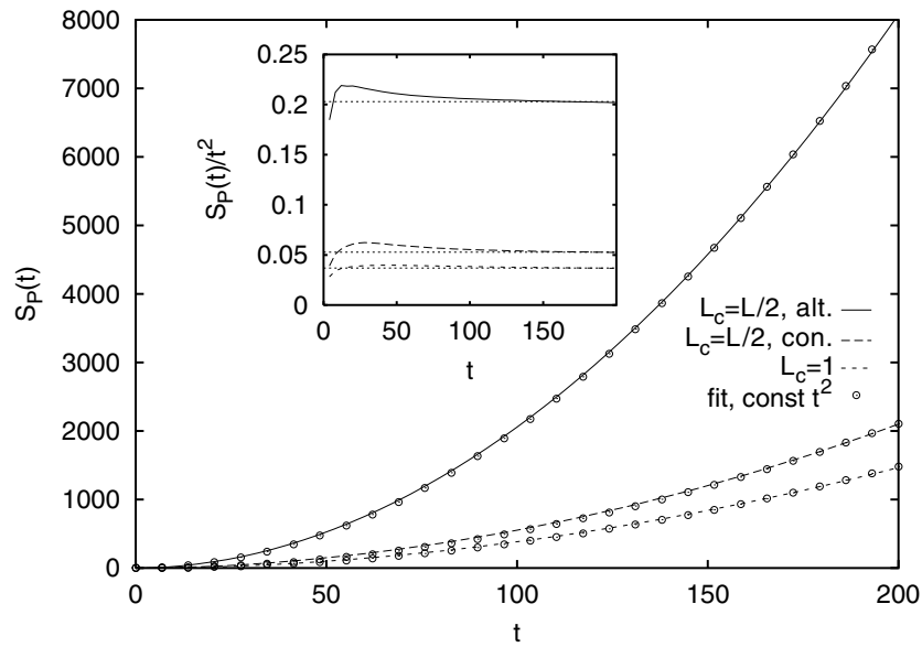
Figure 6. Same as in figure (5) but for the intermediate case (b). Since we have no analytical predictions here, we compare the data by best fitting quadratic functions (sampled symbols—circles and dotted lines in the inset) whose coefficients are later used for comparison to purity fidelity decay.
