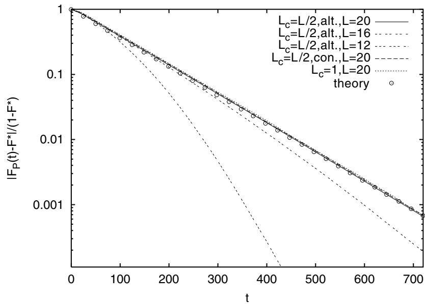
Figure 8. Purity fidelity decay in the mixing regime h_z = 1.4 for different types of division and different sizes L (indicated in the legend) and \delta' = 0.01 . Theoretical decay (for L \rightarrow \infty ) is given by sampled symbols (circles).
