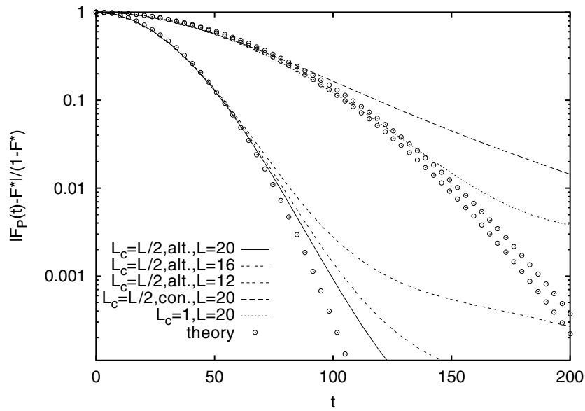
Figure 10. Same as in figure 8 but for the intermediate regime (b).
