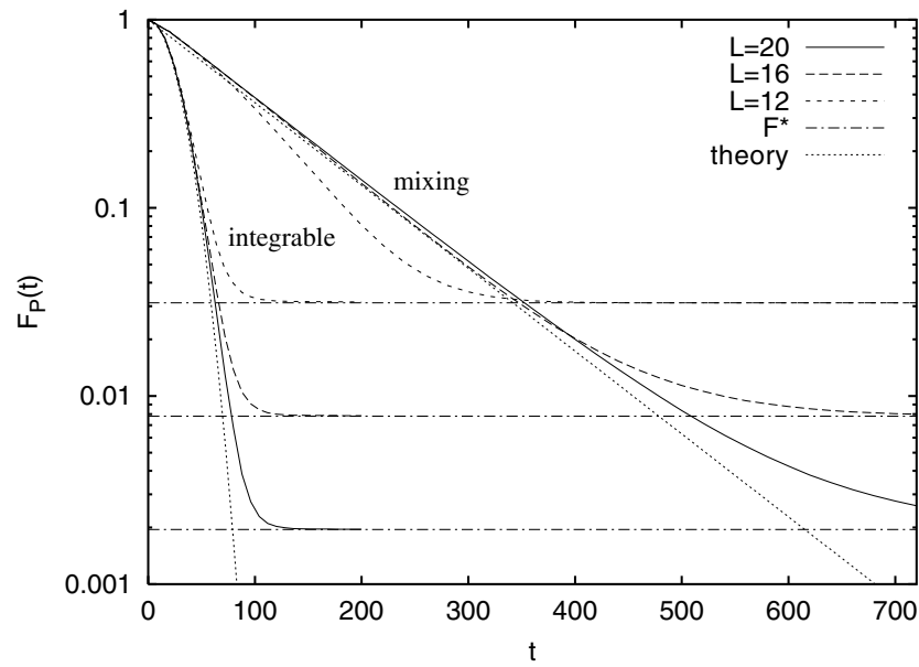
Figure 7. Purity fidelity decay: comparison between mixing h_z = 1.4 and integrable regime h_z = 0 , at scaled perturbation \delta' = 0.01 . Dotted curves give the predicted exponential (26) in the mixing regime and a suggested Gaussian with a theoretically computed timescale (57) in the integrable regime, while horizontal chain lines give the plateau values (34).
