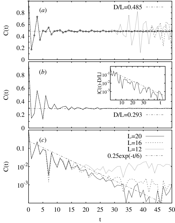
Figure 1. Correlation decay for three cases of KI: (a) integrable h_z = 0 , (b) intermediate h_z = 0.4 and (c) ergodic h_z = 1.4 , for different sizes L = 20, 16, 12 (solid-dotted connected curves, almost indistinguishable in (a) and (b)). Circles (a) show the exact L = \infty result. Chain lines are theoretical/suggested asymptotics (see text).
