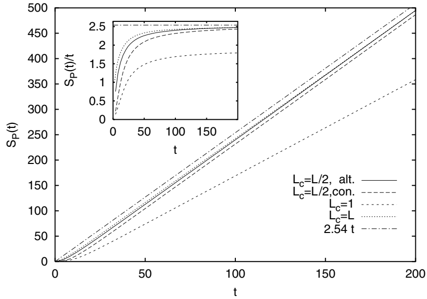
Figure 3. Purity correlator S_P(t) in the mixing regime h_z = 1.4 for different cases (A, C, S and total (non-reduced) correlator, for full, long-dashed, short-dashed and dotted curves, respectively) as compared to the asymptotic linear increase (chain line).
